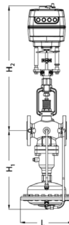
AFQM6 + AME 655, 658 SD
