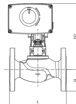
AMV(E) 438, 25, 25 SU/SD, 35 + + VL2 (DN 15–80)
