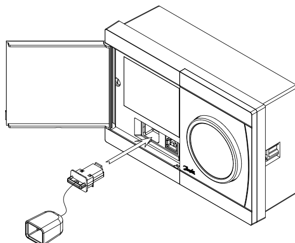
ECL Comfort 296
