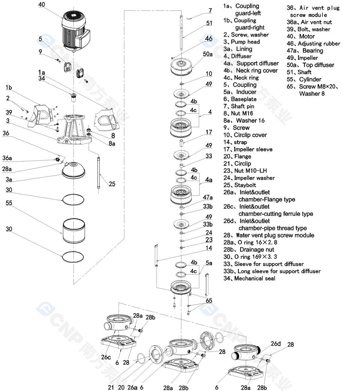
Drawing 1-G CDMF15, 20-240705
