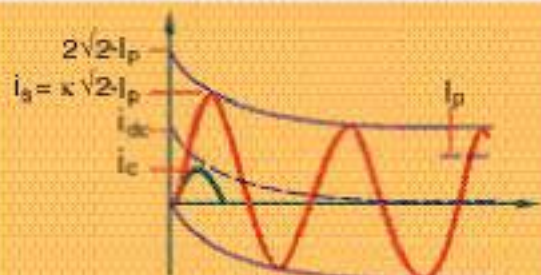
The worst-case scenario for short-circuit current, when provided with a maximum voltage in this phase.
