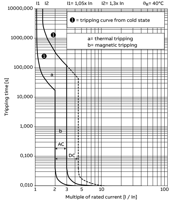
MCB Type S300P - Z (2 ... 3 x I n AC) Tripping Characteristic IEC/EN 60947-2
