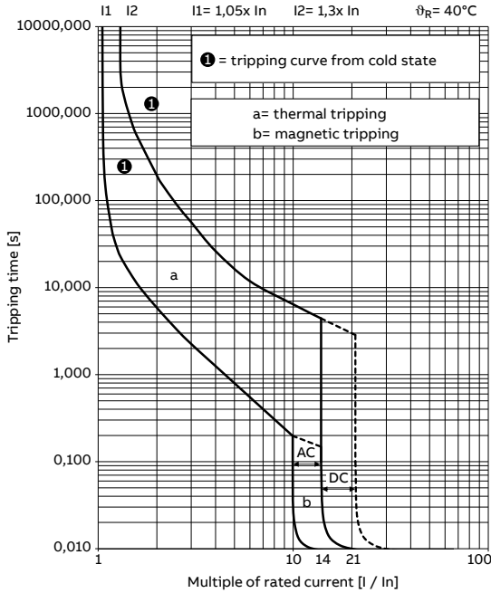
MCB Type S300P - K (10 ... 14 x I n AC) Tripping Characteristic IEC/EN 60947-2
