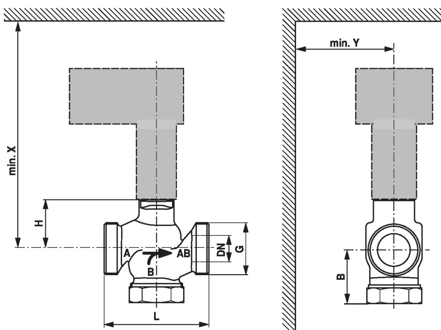
Dimensional drawings
