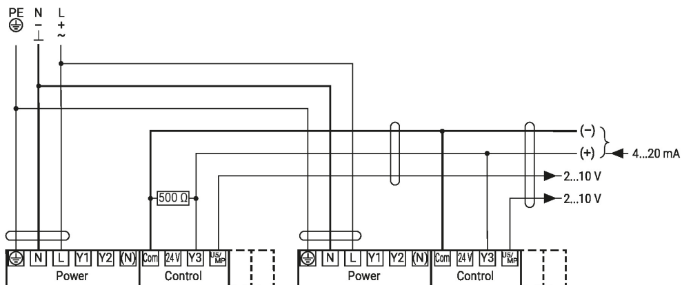
Connection BACnet MS/TP / Modbus RTU with analogue primary/secondary operation
