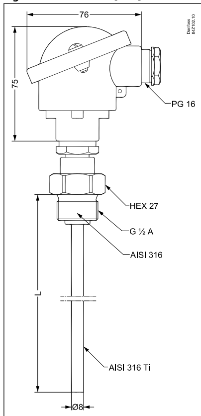
Figure 1: Dimensions [mm]
