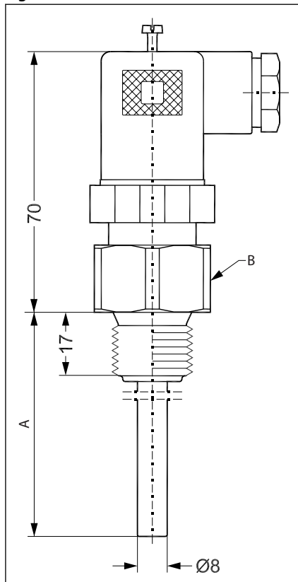
Figure 3: Dimensions
