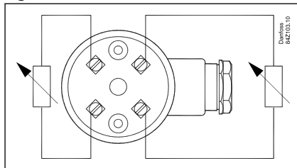
Figure 2: Electrical connection
