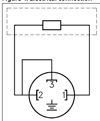
Figure 4: Electrical connection
