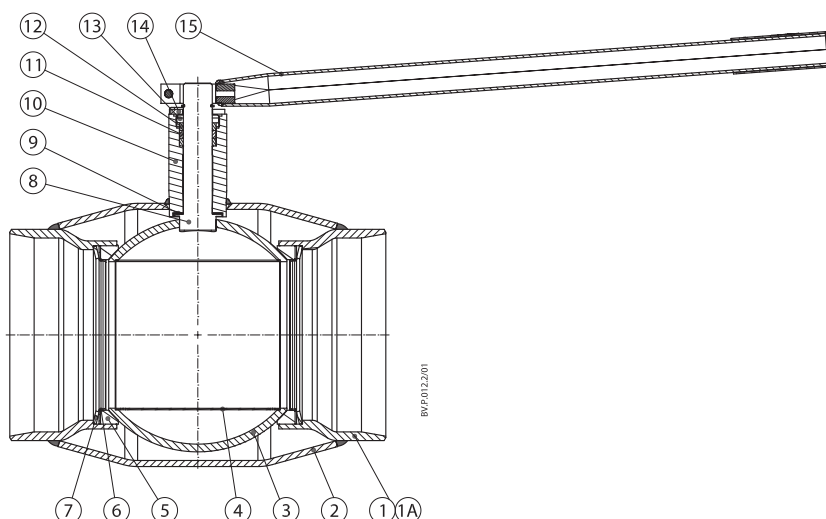
DN 200 with handle
