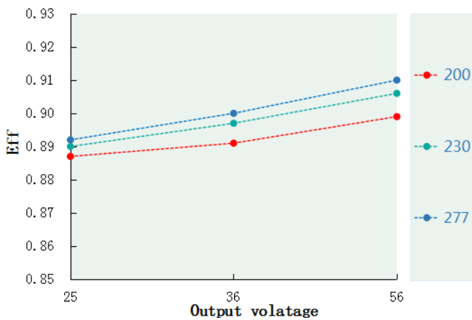
Eff. VS Output voltage DL-100H-56P-MXC
