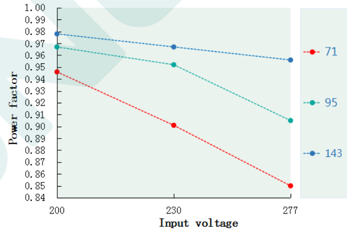
Power factor VS Input voltage DL-100H-143P-MXC
