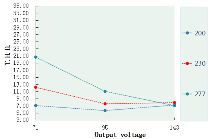
T.H.D. VS Output voltage DL-100H-143P-MXC
