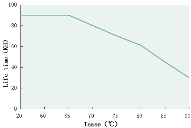
Tcase VS Lifetime(DL-100H-MXC)
