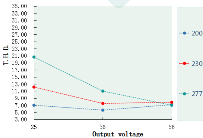
T.H.D. VS Output voltage DL-100H-56P-MXC
