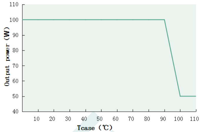
Output power VS Tcase(DL-100H-MXC)
