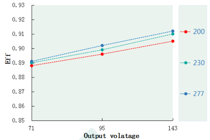
Eff. VS Output voltage DL-100H-143P-MXC
