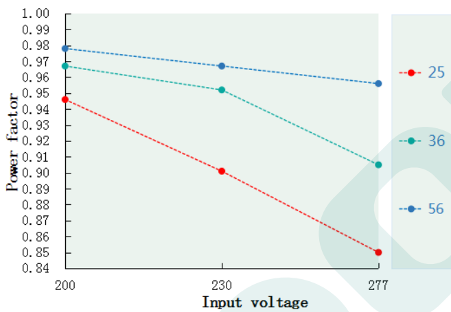
Power factor VS Input voltage DL-100H-56P-MXC
