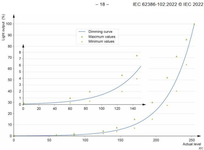
Figure 3 – Dimming curve
