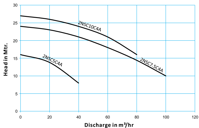
Performance Curves • 2900 RPM
