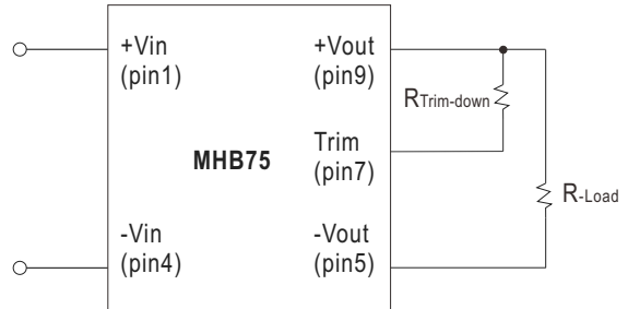
Figure 2 : Trim-down voltage setup
