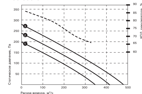
RCS-500-U
