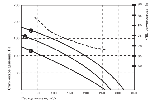
RCS-350-U
