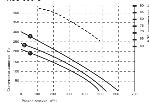
RCS-650-U
