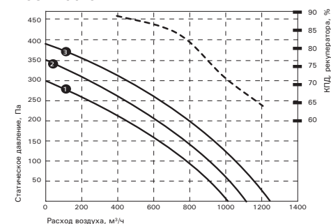
RCS-1250-U
