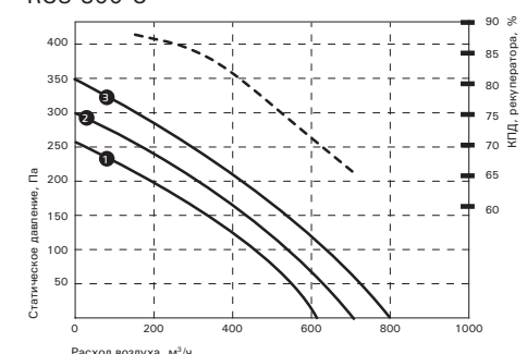
RCS-800-U
