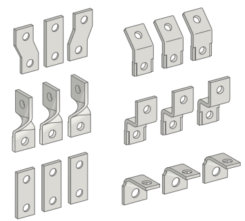
Terminal extensions
