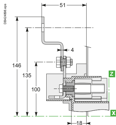
NSX100 to 250
