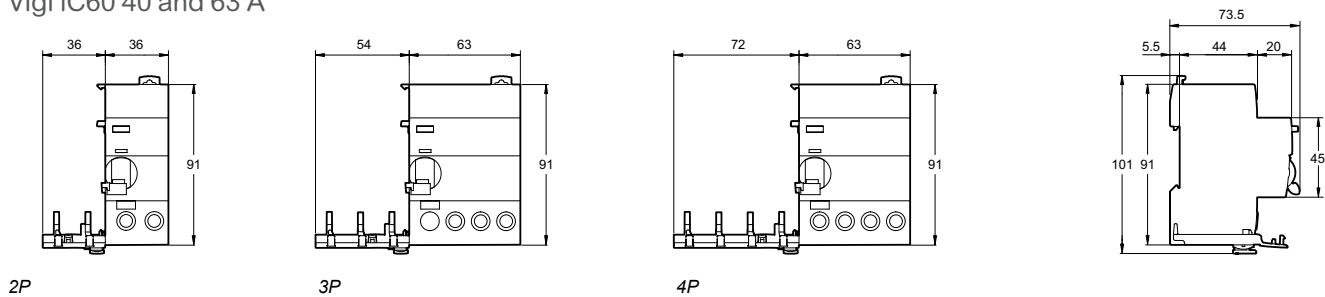
Vigi iC60 40 and 63 A
