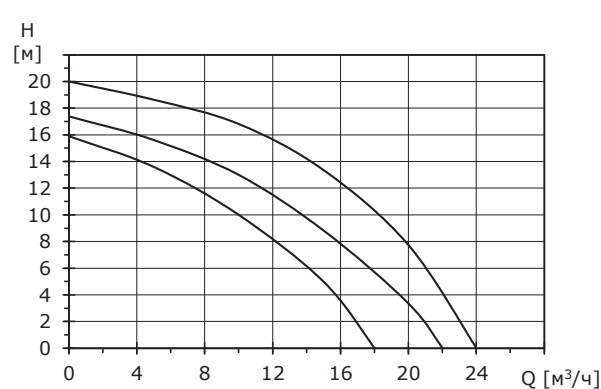
BASIC 50-20SF
