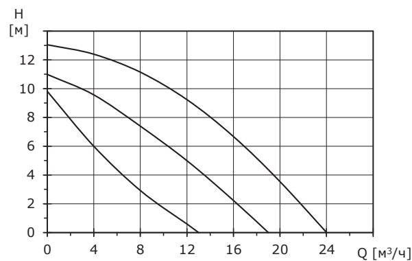
BASIC 50-12SF
