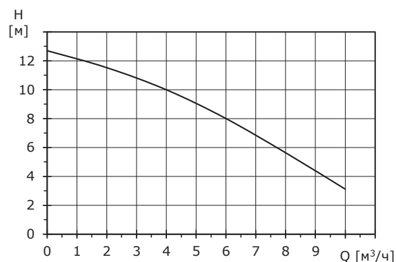
BASIC 32-12F
