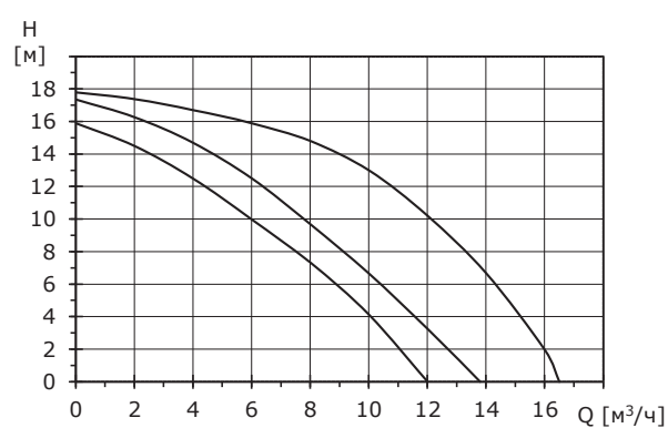
BASIC 40-16SF
