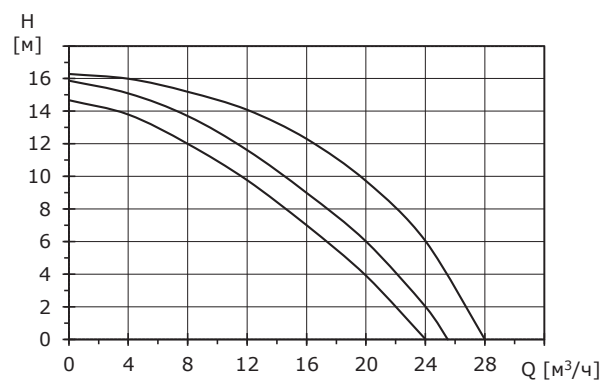
BASIC 50-16SF
