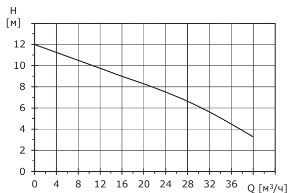
BASIC 65-12F
