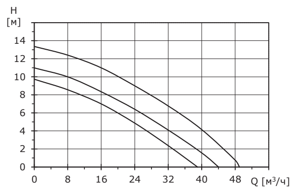
BASIC 65-12SF
