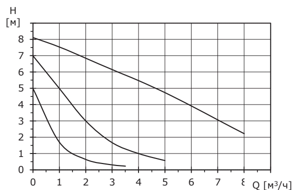
BASIC 32-8SF
