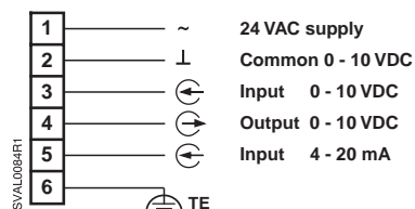
Figure 3. Terminal Layout.
